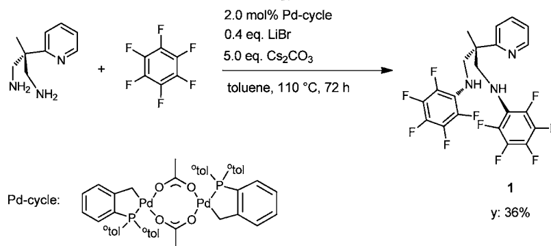
Scheme 1. Synthesis of the Pentafluorinated Ligand \text{H}_2\text{N}_2^{\text{PFPP}}\text{N}_{\text{py}} ( 1 )
