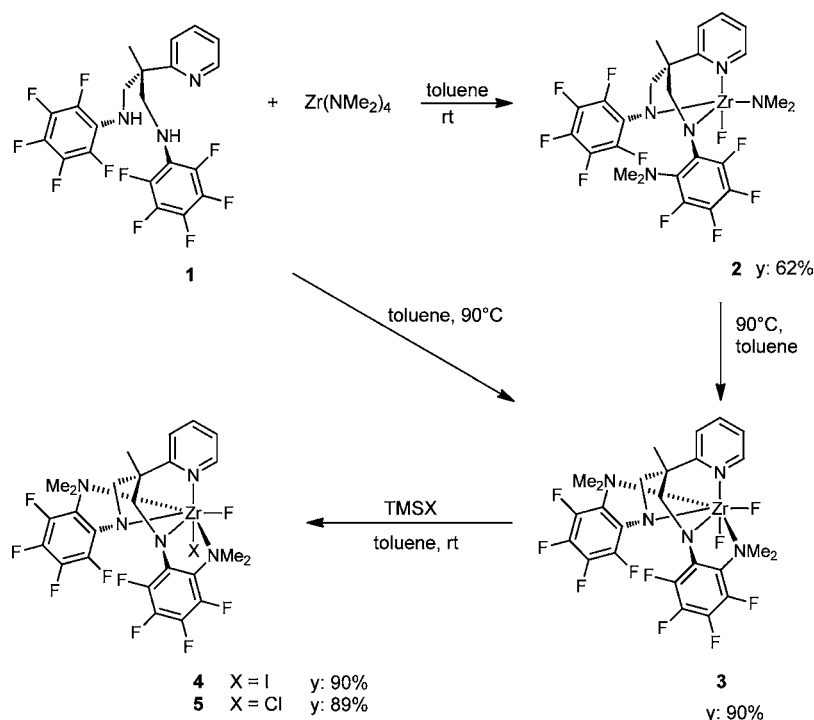
Scheme 2. Ortho Fluorido/Amido Exchange in the Ancillary Diamidopyridyl Ligand 1 upon Reaction with [\text{Zr}(\text{NMe}_2)_4]
